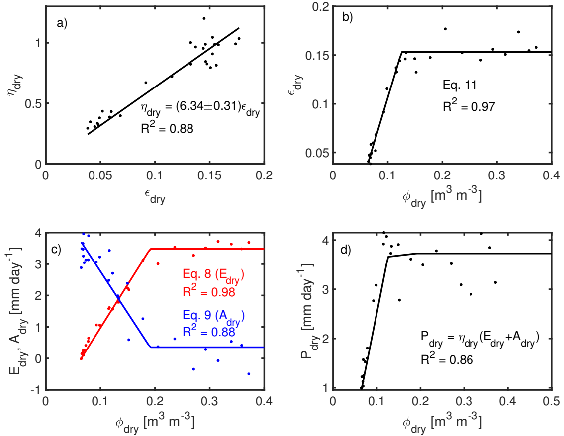
FIG. 9. Conceptual model of P_{\text{dry}} . a) Estimated linear relation between \epsilon_{\text{dry}} and \eta_{\text{dry}} . The estimated coefficient includes a confidence interval of two standard errors. b) Estimated relation between \phi_{\text{dry}} and \epsilon_{\text{dry}} , as given in eq. 11. c) Estimated relations between \phi_{\text{dry}} and E_{\text{dry}} (red line, eq. 8) and A_{\text{dry}} (blue line, eq. 9). d) Predicted relation between \phi_{\text{dry}} and P_{\text{dry}} .
