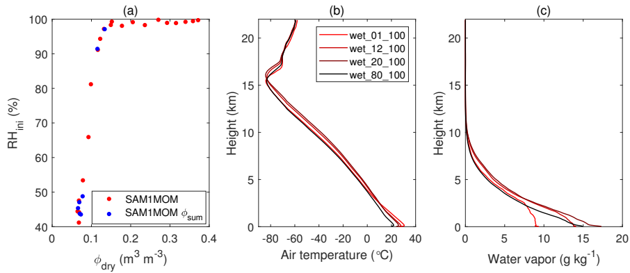
FIG. 3. (a) The initial (6 AM) relative humidity ( RH_{ini} ) at the lowest grid averaged over the whole domain plotted against mean \phi_{dry} in the 1-day simulation. The red dots denote the first 100-day simulations with varying \phi_{dry} but fixed \phi_{wet} , while the blue dots denote simulations with fixed sum of \phi_{dry} and \phi_{wet} . (b) Initial (6 AM) vertical profiles in the 1-day simulations of air temperature and (c) water vapor averaged over the whole domain in the experiments wet_01_100, wet_12_100, wet_20_100, and wet_80_100.
