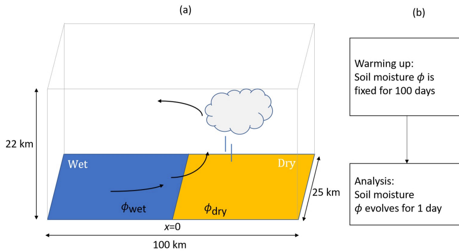
FIG. 1. Schematic of (a) soil moisture setup in the computational domain and (b) two steps of land-atmosphere simulations. \phi_{\text{wet}} and \phi_{\text{dry}} denote soil moisture of the wet patch and dry patch, respectively.
