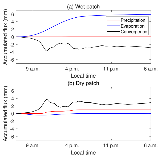
FIG. 6. Accumulated precipitation, evaporation and convergence over the wet (a) and dry (b) patches in the additional 1-day simulation of the experiment wet_01_100.
