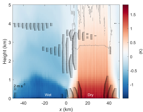
FIG. 5. x - z diagram at 10:00 a.m. local time of y -averaged quantities for additional 1-day simulation of the experiment wet_01_100. The color contours denote temperature anomaly. The black arrows denote zonal velocity with absolute values not less than 2 \text{ m s}^{-1} , and the text “ 2 \text{ m s}^{-1} ” in the bottom left of the figure denotes the velocity of the arrow below. The grey isolines denote non-precipitating cloud ice and water equal to 10^{-5} \text{ g kg}^{-1} . The x axis denotes the distance from domain center in x direction.
