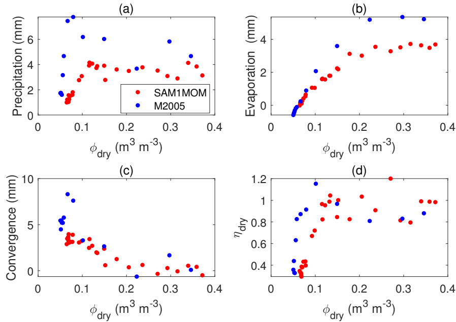
FIG. 7. Accumulated precipitation, evaporation, convergence, and large-scale precipitation efficiency \eta_{\text{dry}} over the dry patch in the additional 1-day simulation of the experiments. The red dots denote experiments using the microphysics scheme SAM1MOM, and the blue dots denote experiments using the microphysics scheme M2005.
